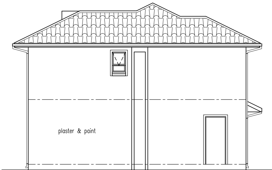
WEST ELEVATION (1:100)
