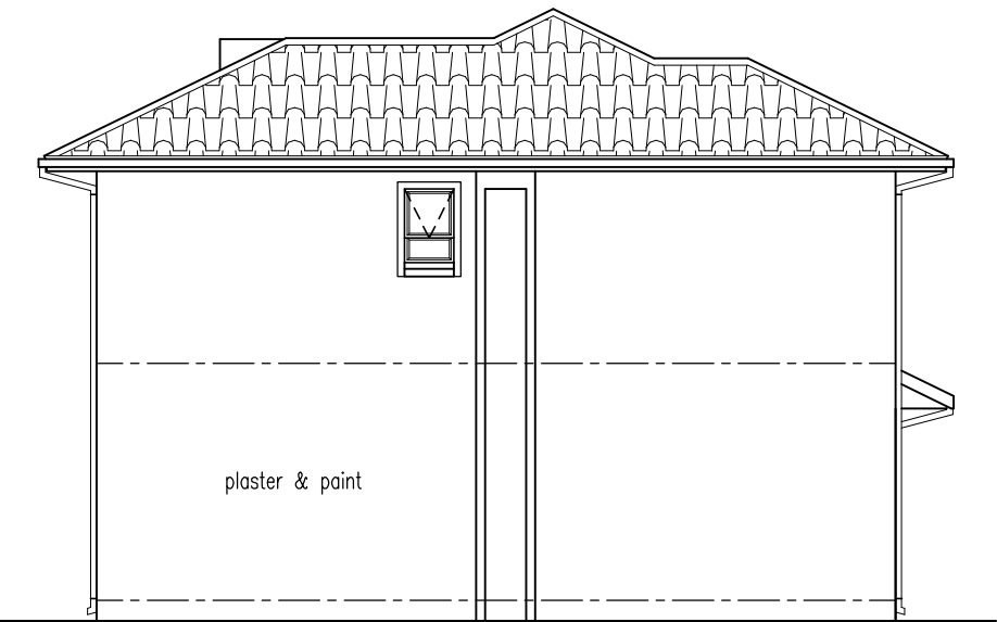
WEST ELEVATION (1:100)
