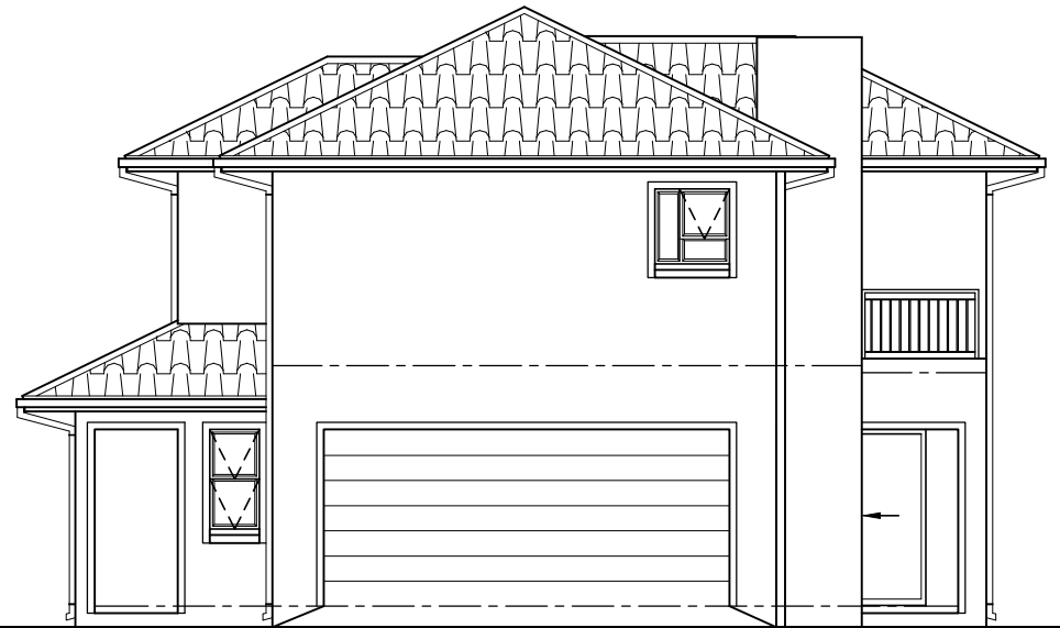
EAST ELEVATION (1:100)
