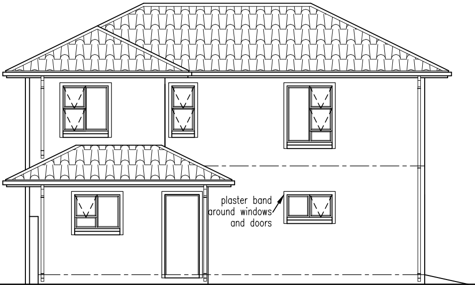
SOUTH ELEVATION (1:100)
