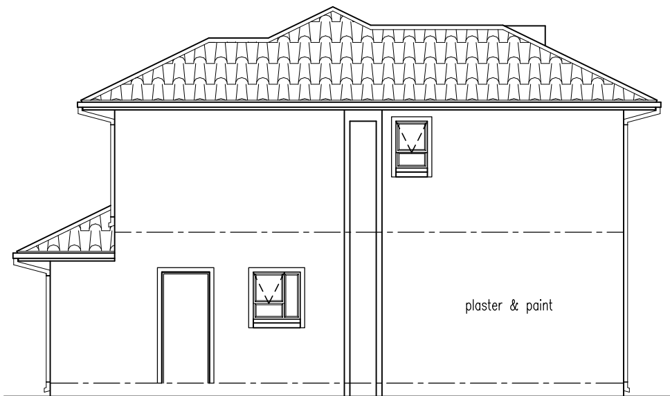
EAST ELEVATION (1:100)
