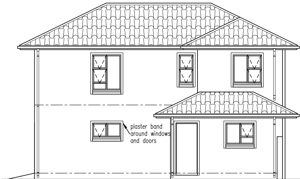
SOUTH ELEVATION (1:100)
