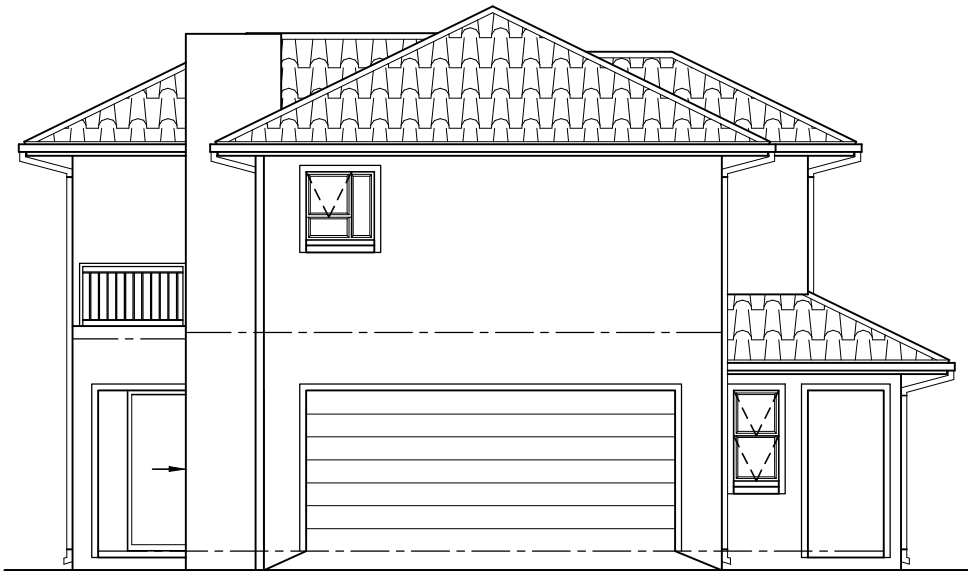
WEST ELEVATION (1:100)
