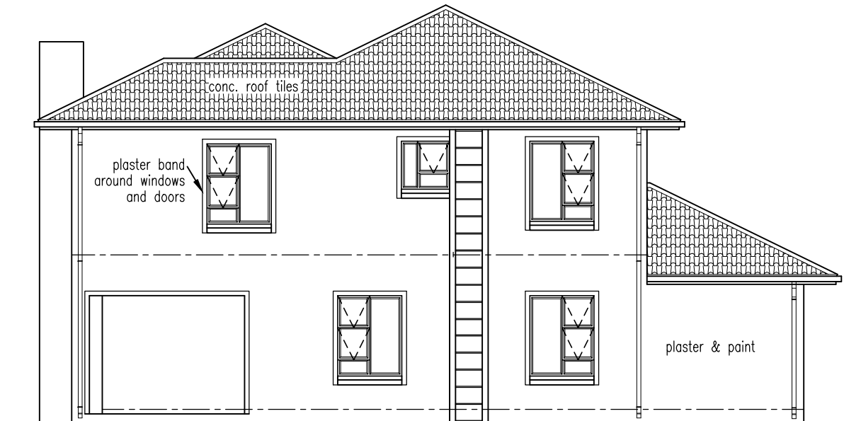
NORTH ELEVATION (1:100)
