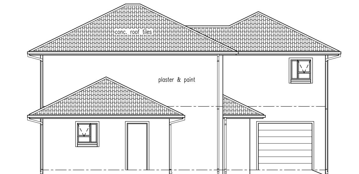
WEST ELEVATION (1:100)
